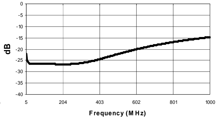
Isolation
