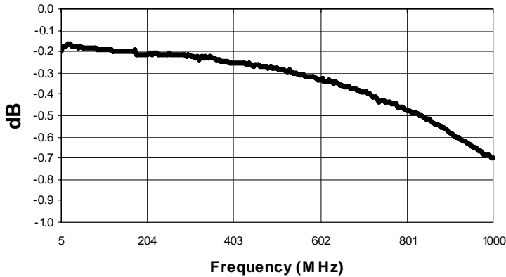
Insertion Loss
